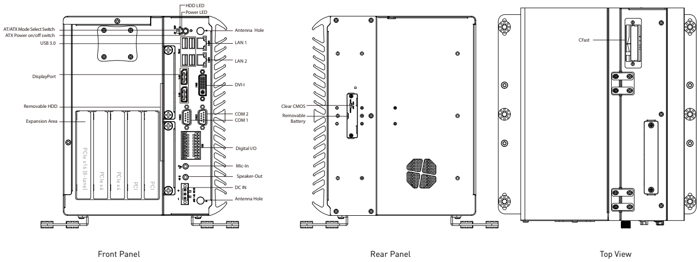
Front Panel
