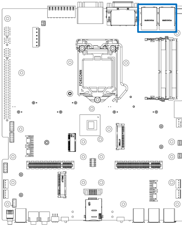
LAN1 LAN2 USB3.2 GEN 2 x4 Ports
