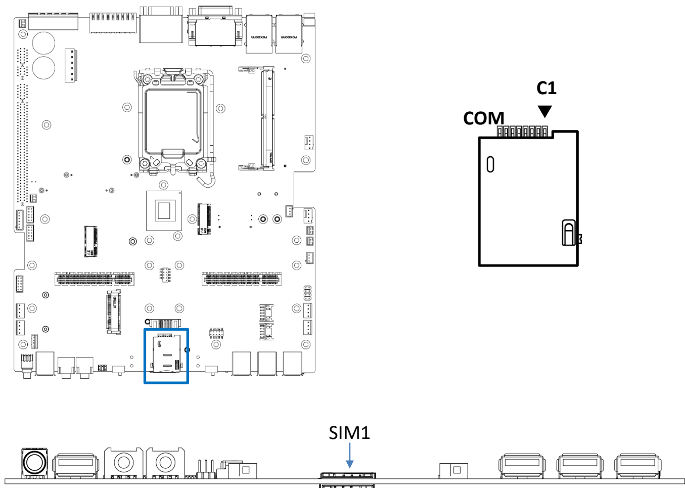
SIM1 (Top size for M.2 B Key)
