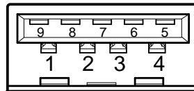
USB3_1 : USB3.1 Connector, Type A
