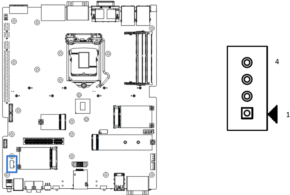
PWR_SW3 : Remote Power Switch 1x4 pin box header, 2.0mm pitch
