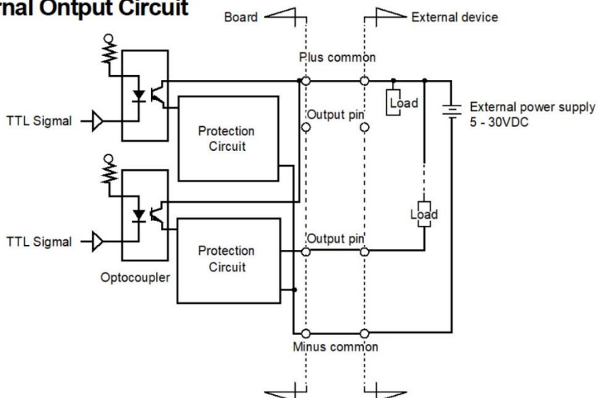
External Output Circuit
