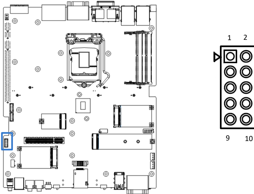
CN7 : USB3.0 Connector 2x5 9-pin header, 2.0mm pitch
